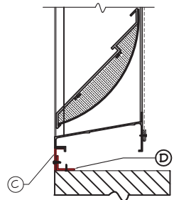
FLANGE W/ SUBFRAME
