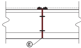
VERTICAL SEMI-INVISIBLE MULLION
