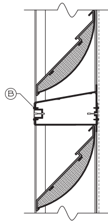
HORIZONTAL VISIBLE MULLION
