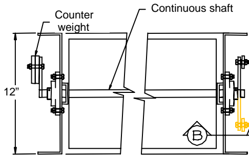
Section - C
