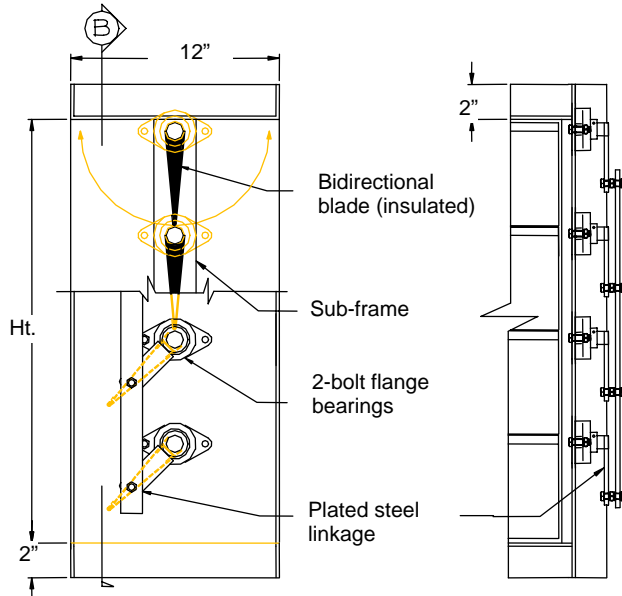
Section - B
